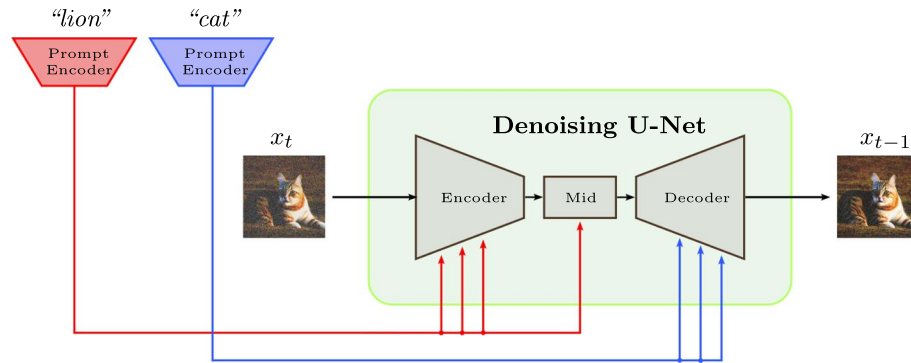
Fig. 6 USPLIT pipeline illustration. Encoder+bottleneck blocks (red) receive p_1^* , while decoder blocks (blue) receive p_2^* . This often retains the shape of the first concept and overlays stylistic details from the second
