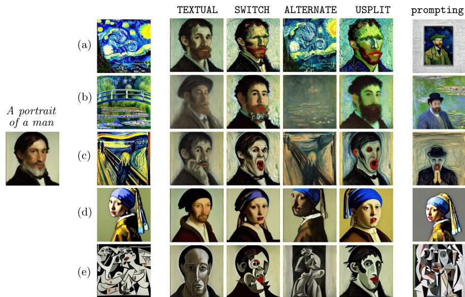
Fig. 12 Style blending examples for the main concept “A portrait of a man”, combined with a “ Starry Night by van Gogh”, b “ Water Lilies by Claude Monet”, c “ The Scream by Edvard Munch”, d “ Girl with a Pearl Earring by Johannes Vermeer”, and e “ Guernica by Pablo Picasso”. The last column shows the baseline result using a single “in the style of” prompt. All images are generated with the same random seed
