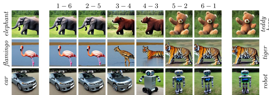
Fig. 7 Qualitative results for the USPLIT method. Each row uses different prompt pairs (e.g., “elephant” vs. “teddy bear”), and columns labelled n - m show different split choices, where the first n blocks use p_1^* and the last m blocks use p_2^* . The analysis provides insights into which split generates better results. All variants are generated with the same random seed to isolate the effect of the split
