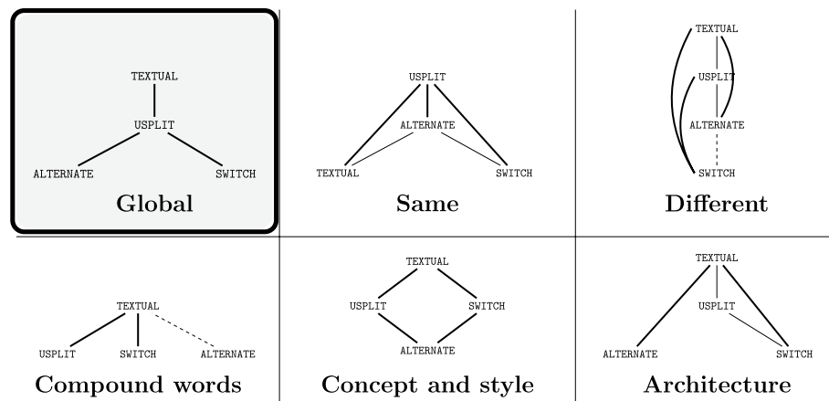
Fig. 16 Ordering preferences by category. In the Hasse diagrams, thick lines mean extremely significant (p-value < 0.001), thin lines mean very significant (p-value < 0.01) and dashed lines mean significant (p-value < 0.05)
