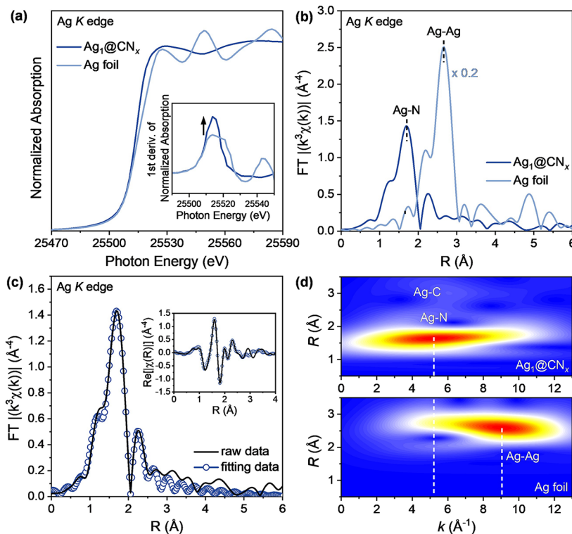
Figure 3. X-ray absorption spectroscopy data of Ag K edge for \text{Ag}_1@\text{CN}_x and Ag foil. (a) Ag K edge XANES spectra, (b) non-phase corrected k^3 -weighted FT-EXAFS spectra, (c) EXAFS fitting data for \text{Ag}_1@\text{CN}_x , and (d) corresponding WT-EXAFS data.
