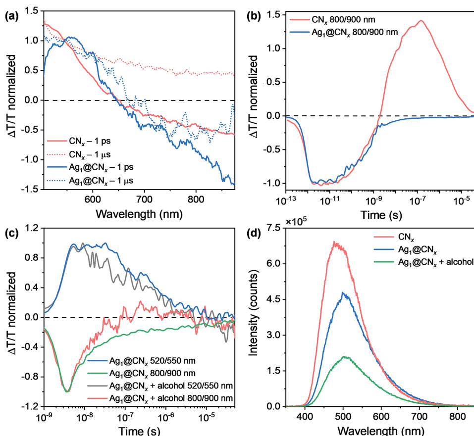
Figure 6. (a) Transient absorption spectra at 1 ps (solid line) and 1 \mu s (dashed line) after photoexcitation of \text{CN}_x (red line) and \text{Ag}_1@\text{CN}_x (blue line). (b) Dynamics probed at 800–900 nm from \text{CN}_x (red line) and \text{Ag}_1@\text{CN}_x (blue line), and (c) dynamics collected from \mu s-TA in the 520/550 and 800/900 nm spectral range on \text{Ag}_1@\text{CN}_x in acetonitrile, with and without the addition of benzyl alcohol (37 \text{mmol L}^{-1} ). As evidenced, the sample with benzyl alcohol shows a faster decay of both the PIA (green and red line) and PB (black and blue) signals compared to the counterpart without substrate, suggesting an efficient carrier extraction from the scaffold to the reactant. (d) Comparison of static photoluminescence spectra of \text{CN}_x and \text{Ag}_1@\text{CN}_x , with and without the addition of benzyl alcohol (37 \text{mmol L}^{-1} ). The intensity of the signal is quenched with the introduction of benzyl alcohol due to the extraction of a part of the photoexcited carriers.
