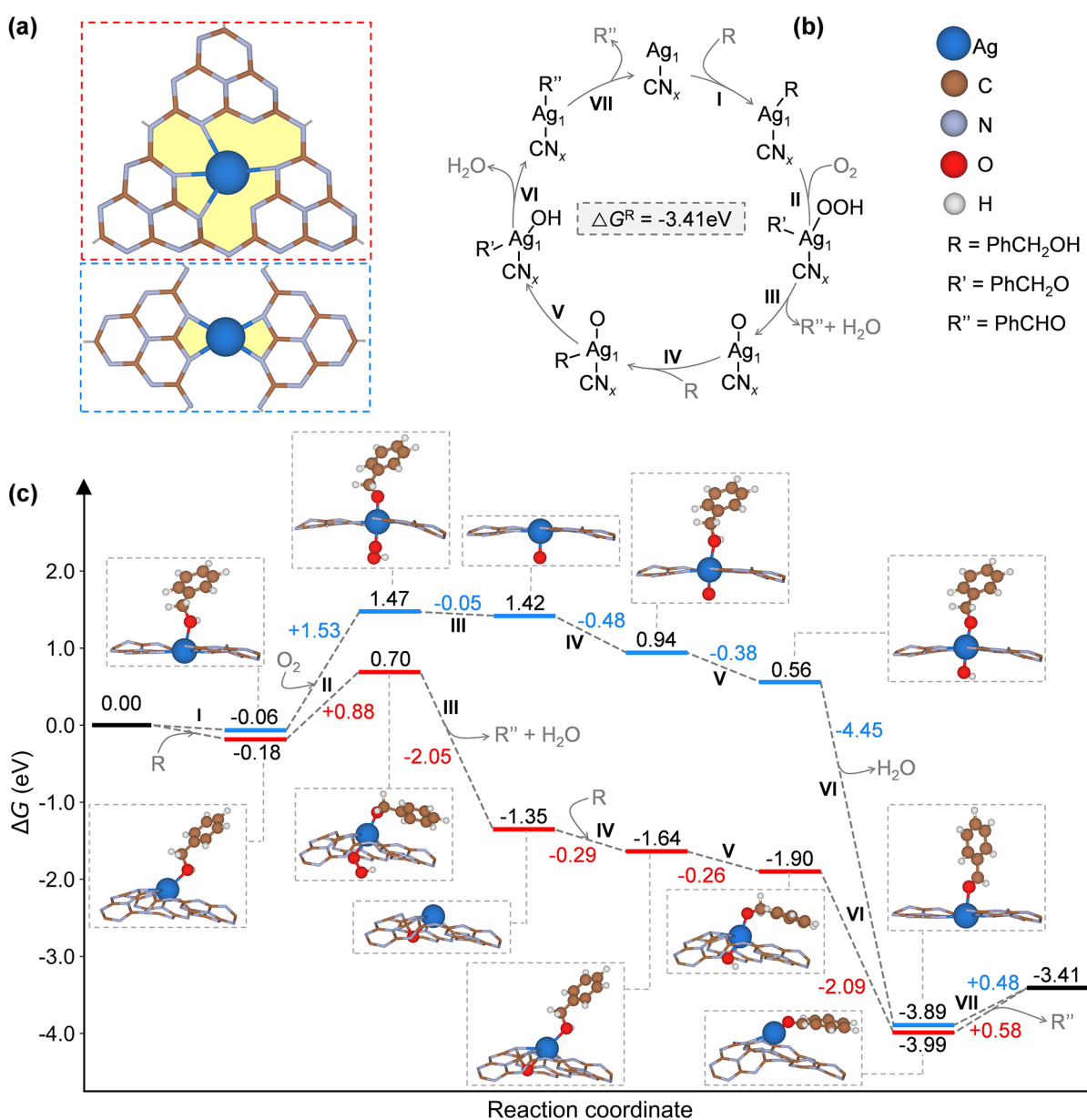
Figure 7. (a) Atomistic structure of Ag atom in the heptazine pore of CN_x (top, red dotted line) and the pore of the new structure of CN_x (bottom, blue dotted line), (b) mechanism of the oxidation of benzyl alcohol to benzaldehyde, and (c) Gibbs free energy profile for the oxidation of benzyl alcohol to benzaldehyde. Brown, blue, light purple, red, and white balls correspond to carbon, silver, nitrogen, oxygen, and hydrogen atoms. In the figures the roman numbers indicate the elementary steps of the process.
