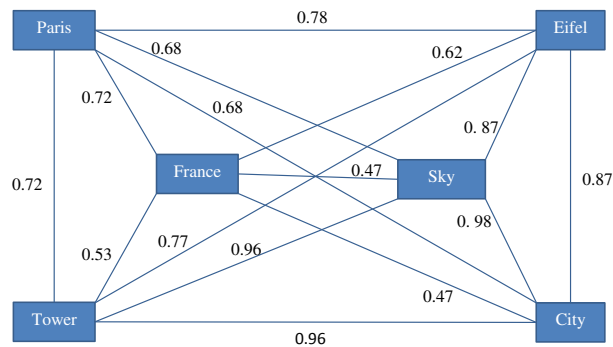
Figure 3. Similarity graph for the data points corresponding to the rows of the matrix shown in Figure 2. The nodes corresponds to the tags with edges weighted using the cosine similarity
