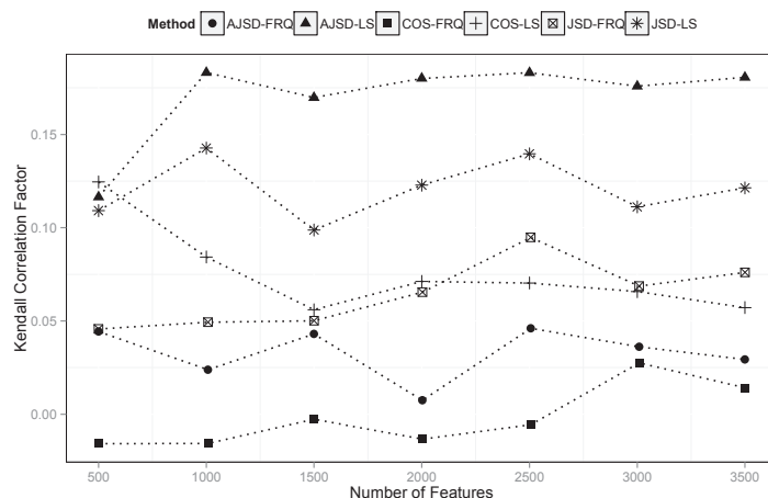
Figure 8. Kendall \tau correlation achieved AJSD, JSD and COS. These measure are investigated using LS feature selection and the FRQ method and using increasing number of features
