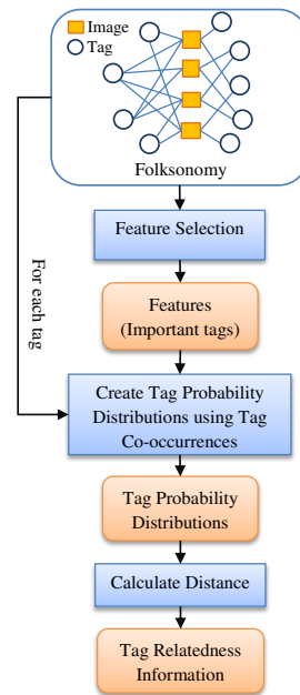
Figure 1. The workflow of the proposed tag relatedness approach
