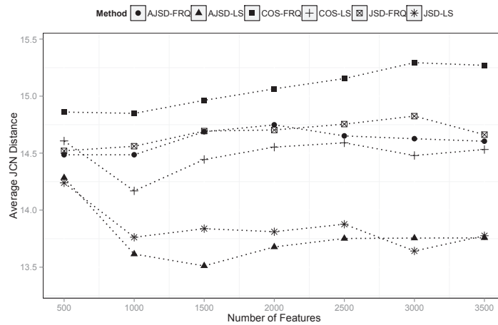
Figure 7. Average JCN achieved AJSD, JSD and COS. These measure are investigated using LS feature selection and the FRQ method and using increasing number of features
