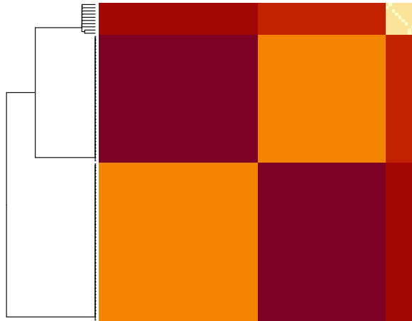
Figure 11: Dissimilarity matrix returned by partition(fit.sim) , obtained by using Wade and Ghahramani (2018) 's method with variation of information loss function ( dist = "VI" ).
