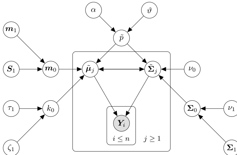
Figure 4: Hierarchical representation of the multivariate PY process mixture model with location-scale base measure and full covariance matrix.
