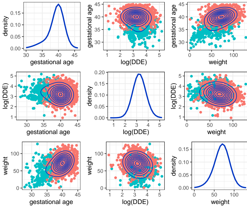
Figure 10: Posterior mean densities, univariate marginal and pairwise bivariate marginal, obtained by calling plot() on the fitted model fit2 . In addition to the posterior mean density value, each pairwise bivariate density shows the data points colored according to the estimated clustering.
