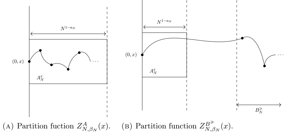
FIGURE 1. The above figures depict the chaos expansions of Z_{N,\beta_N}^A(x) and Z_{N,\beta_N}^{B \geqslant}(x) . The disorder sampled by Z_{N,\beta_N}^A(x) is restricted to the set A_N^x , while that of Z_{N,\beta_N}^{B \geqslant}(x) is restricted to B_N^{\geqslant}
