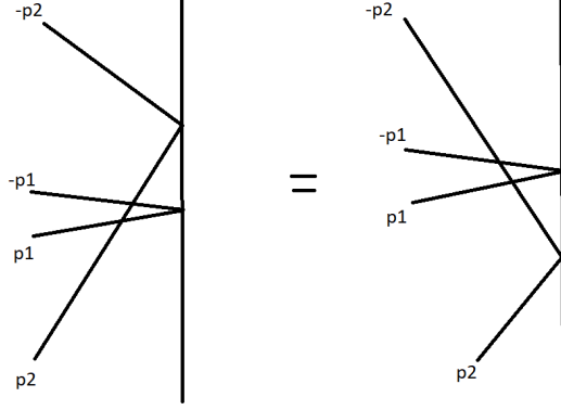
Figure 1: The Boundary Yang-Baxter Equation (BYBE) for a right wall (hence all the incoming particles are right movers, and all the outgoing particles after reflection are left movers).
