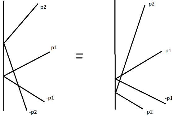
Figure 3: The Boundary Yang-Baxter Equation (BYBE) for a left wall (hence all the incoming particles are left movers, and all the outgoing particles after reflection are right movers).
