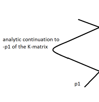
Figure 2: The unitarity condition for the right wall. One has to analytically continue the expression for the reflection matrix (which is defined for positive incoming momentum) to negative incoming momentum (a left mover is fed back into the right wall).
