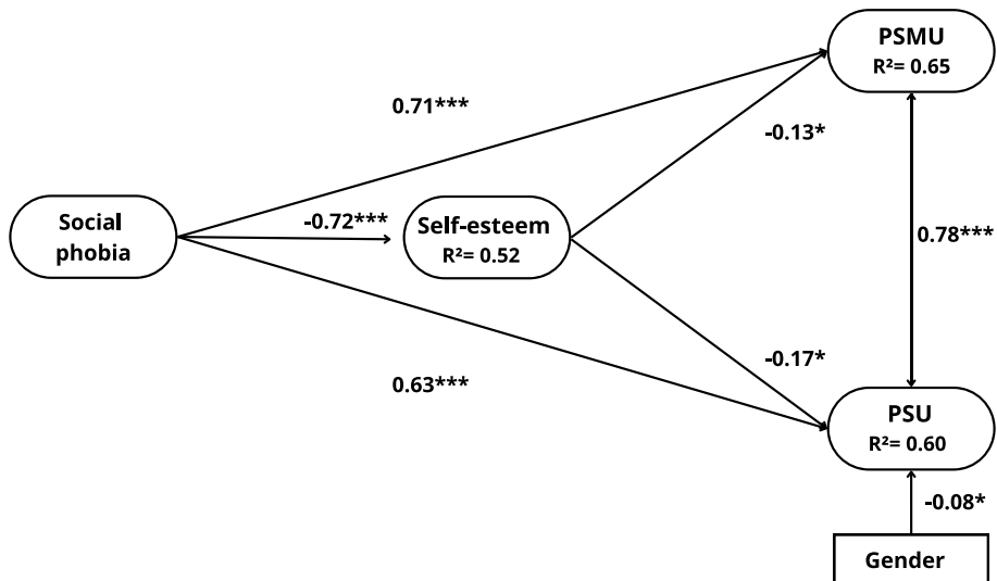
Fig. 2 Standardized results of the SEM model. The latent factors are presented in an oval. Covariate (Gender dummy coded - 1=male, 2=female) is represented in a rectangle. Item factor loadings, significant at p<0.001 , are omitted. PSU=problematic smartphone use; PSMU=problematic social media use. Non-significant path is omitted. * p<0.05 , ** p<0.01 , *** p<0.001
