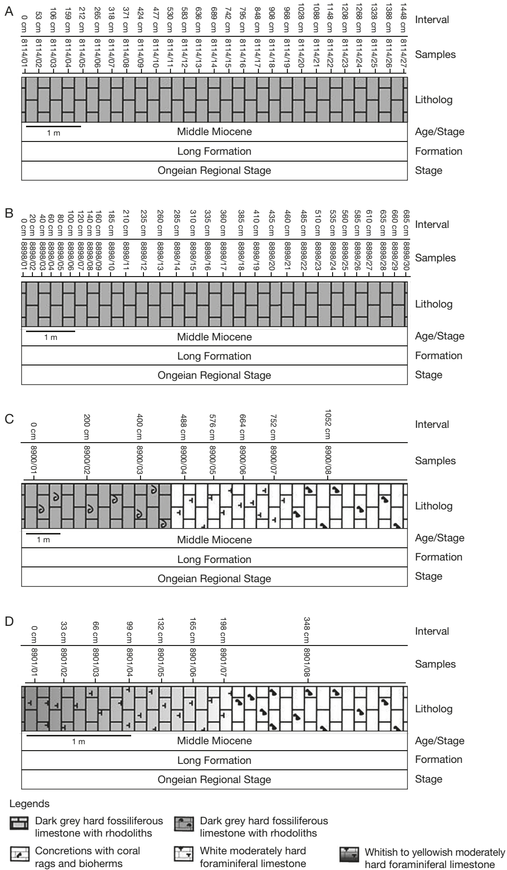
FIG. 2. — Lithologies of the outcrops: A , Butler Bay Section-I; B , Butler Bay Section-II; C , Hut Bay Quarry No. 4 Section; D , New Quarry Section.
