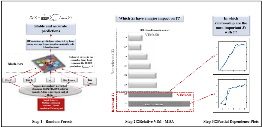
Figure 1. Three-step procedure based on Random Forest, VIM and PDP
