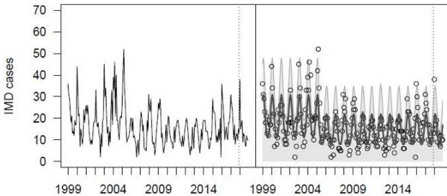
Figure 1. Left panel: Time series of the monthly number of invasive meningococcal disease (IMD) cases in Italy for the years 1999–2018. Right panel: observed ( \circ ) and predicted (—) number of IMD cases. The vertical dotted line separates the data used for model fitting from the data used for the prediction exercise.
