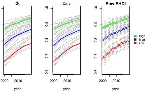
Figure 1. Cluster centroids: k-means with different distances.
