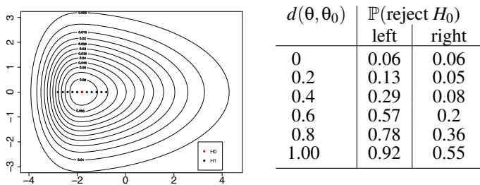
Figure 1. Contour plot of a density and associated estimated Type I error probability for a nominal \alpha = 0.05 and power for increasing distance from H_0 .
