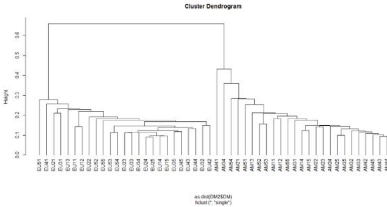
(b) Squared returns levels.
