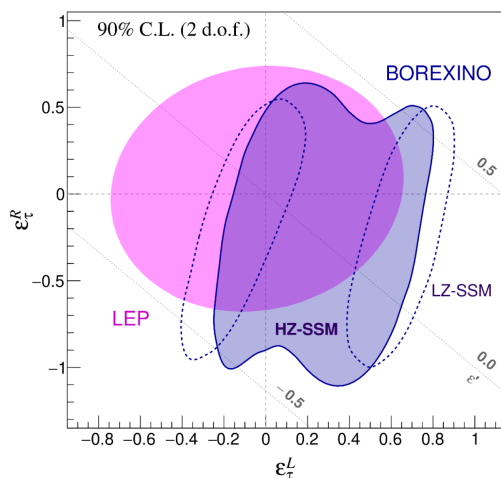
Fig. 6. Allowed region for NSI parameters in \epsilon_\tau^{L/R} plane obtained in. 29 The \epsilon_e^{L/R} are fixed at zero. Both HZ- (filled dark blue) and LZ- (dashed dark blue) SSM's are considered. The contour from LEP experiment is provided for comparison. Both contours correspond to 90% C.L. (2 d.o.f.). The dotted gray lines represent the corresponding range of \epsilon_e^{L/R} parameter, relevant for NSI's at propagation.
