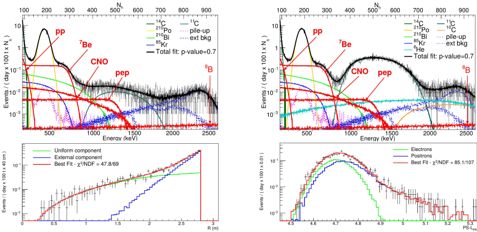
Fig. 4. Result of the simultaneous measurement of low-energy pp -chain solar neutrinos. Top panel: visible energy spectra in the ^{11}\text{C} -subtracted (left) and -tagged datasets. Bottom left: Distribution of the events distance from the detector centre. Bottom right: Distribution of the pulse shape parameter. All figures from. 14
