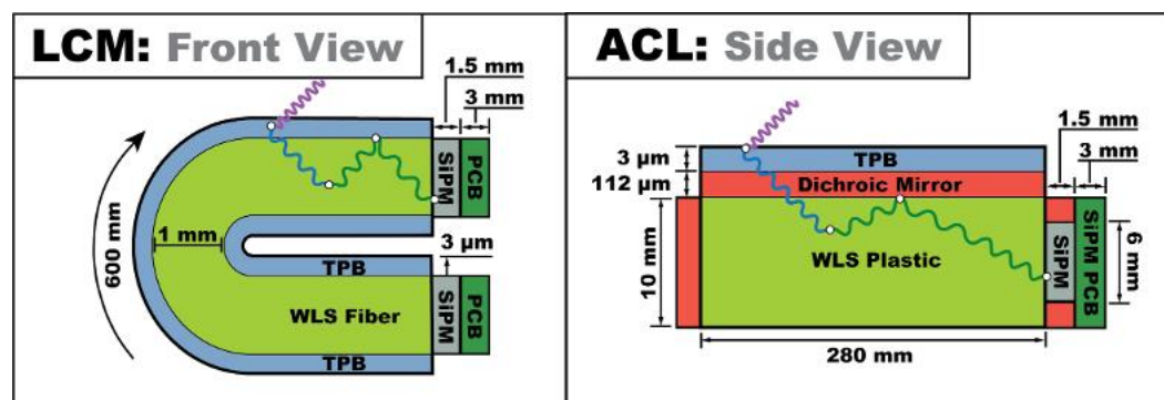
Figure 5. Schematics of the two LRS light trap types deployed in the 2x2 Demonstrator: the LCM (left) and ACL (right) with their respective dimensions. Installed in the detector, individual LCMs measure 10 cm vertically, while a single ACL spans 30 cm along the same dimension. The oscillating lines represent possible photon trajectories, with interactions at each white point shifting the 128 nm scintillation light to a more easily detected 512 nm (green).
