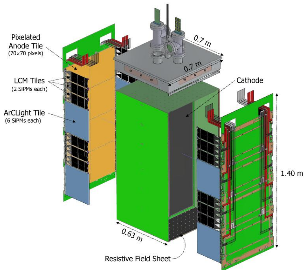
Figure 4. Rendering of a single 2x2 module, as described in [8]. The module is bisected by a resistive cathode to form two optically isolated LArTPCs. Readout cable positions for the CRS (gray) and LRS (red) can be clearly seen external to the anode. During operation, modules are protected by an external G10 sleeve.
