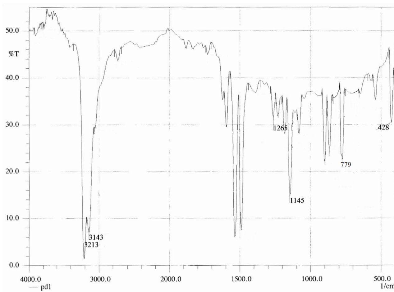
Figure 3. Experimental IR spectrum of the [\text{Pd}(\text{CPDA})\text{Cl}_2] complex.
