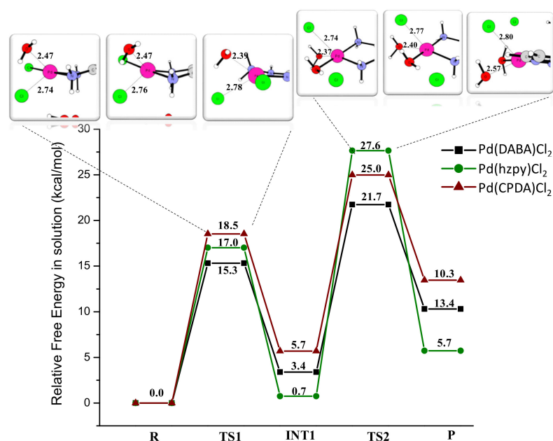
Figure 12. Potential energy profiles for the first and second hydrolysis reaction of the investigated Pd(II) complexes, with snapshots of the first and second transition states (TS1 and TS2), computed in water at the B3LYP/6-31++G(2df,2pd)/SDD-level of theory. The reactants, first intermediate and product of the reaction are referred as R, INT1 and P in the energetic profile, respectively. More details can be found in SI section.
