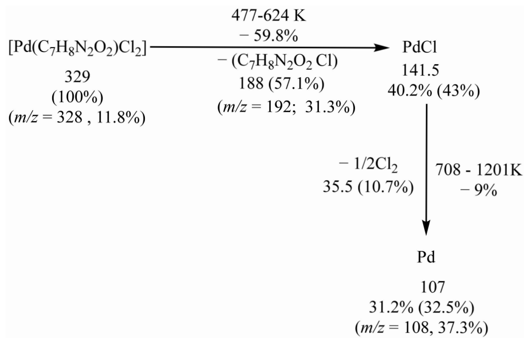
Scheme 1. Thermal decomposition of the [Pd(DABA)Cl 2 ] complex.
