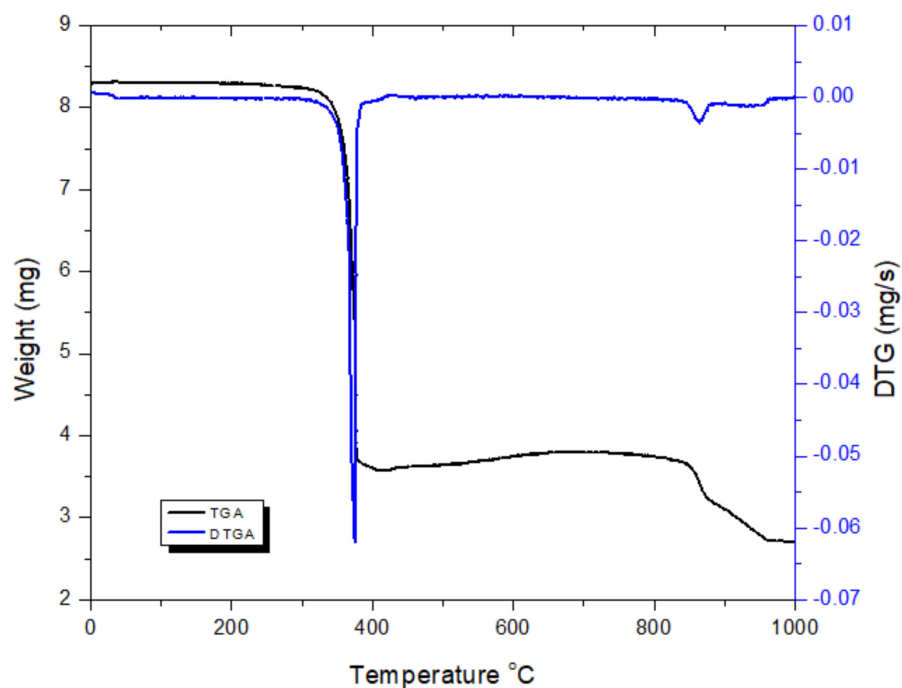
Figure 5. Thermogram of the [Pd(DABA)Cl 2 ] complex (TG: black; DTG: blue).
