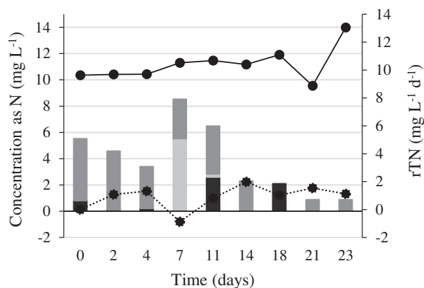
Figure 3. Total inorganic nitrogen (TN) concentration in the influent (solid line), N compounds in the effluent (bars, NH_4^+ -N in black, NO_2^- -N in light grey and NO_3^- -N in dark grey) and nitrogen removal rate (rTN; dashed line) detected in the PBR over time.
