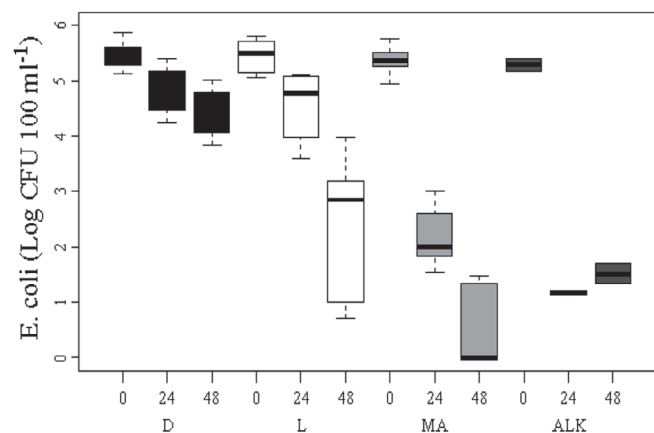
Figure 1. Counts of E. coli detected in the different batch tests at time 0 and after 24 and 48 h. D (black blocked boxes) are the tests kept in the dark without the microalgae, L (white blocked boxes) are the tests kept illuminated without the microalgae, MA (light grey blocked boxes) are the tests which were inoculated with microalgae and kept under light, ALK (dark grey blocked boxes) are the tests in which the pH was adjusted to 12 and kept under light.
