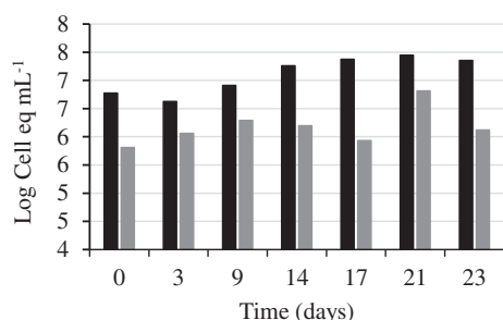
Figure 7. Concentration of total bacteria in the influent (black bars) and in the effluent (grey bars) of the PBR detected over time.
