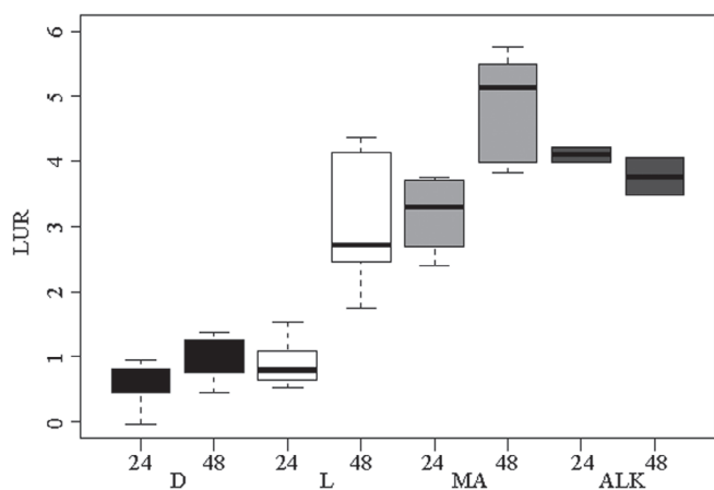
Figure 2. Logarithmic unit removal (LUR) of E. coli in the batch tests after 24 and 48 h. D (black blocked boxes) are the tests kept in the dark without the microalgae, L (white blocked boxes) are the tests kept illuminated without the microalgae, MA (light grey blocked boxes) are the tests which were inoculated with microalgae and kept under light, ALK (dark grey blocked boxes) are the tests in which the pH was adjusted to 12 and kept under light.
