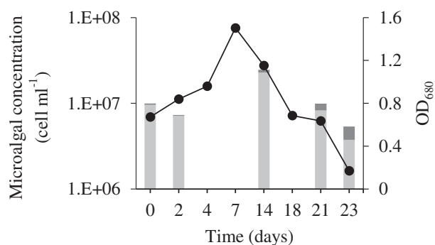
Figure 4. Distribution of the main algal species ( Chlorella spp. in light grey, Scenedesmus spp. in dark grey and Chlamydomonas spp. in black) and algal density expressed at OD_{680} (solid line) detected over time in the PBR. Data of microalgal number at days 4, 7 and 18 are not available.
