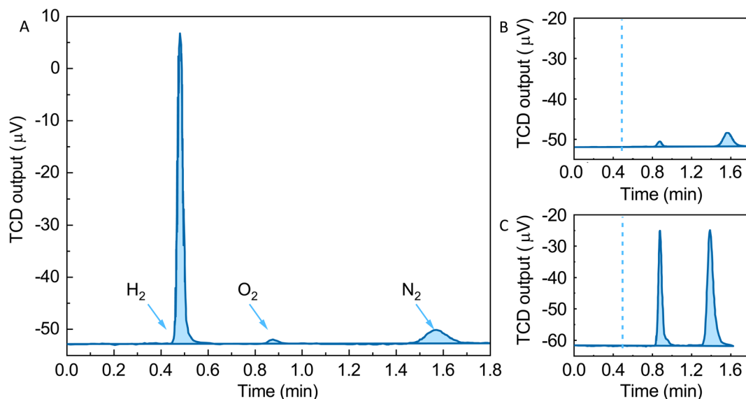
Fig. 2 GC traces corresponding to the atmosphere of sealed vials containing: (A) N-DMBI-H:P(NDI2OD-T2) 2:1 blend; (B) pure N-DMBI-H; (C) pure P(NDI2OD-T2). Light blue arrows indicate peaks corresponding to H 2 , O 2 and N 2 in (A). H 2 retention time is highlighted with a light blue dashed line in (B) and (C).
