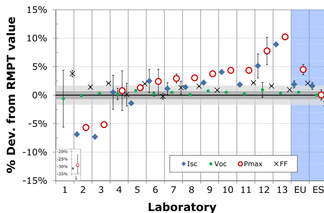
FIGURE 5 Percentage deviations from ESTI RMPT value for I_{\text{SC}} , V_{\text{OC}} , P_{\max} and FF of RR83 (a-Si/ \mu\text{c-Si} ). RMPT value is represented by the x-axis, and its combined expanded UC ( k = 2 ) is shown for simplicity only for P_{\max} (light-grey-shaded area) and FF (dark-grey-shaded area). The error bars shown represent the UC of the submitted result as stated by the participant. The EU and ES values correspond to the ESTI measurements made, respectively, before and after the pre-conditioning at the end of the RR PT. An inset is shown for the points falling outside the main range of the deviations. Note that the laboratory identification number may be different for the other DUTs [Colour figure can be viewed at wileyonlinelibrary.com ]
