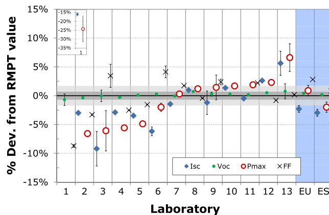
FIGURE 6 Percentage deviations from ESTI RMPT value for I_{SC} , V_{OC} , P_{max} and FF of RR84 (a-Si/ \mu c-Si). RMPT value is represented by the x-axis, and its combined expanded UC ( k = 2 ) is shown for simplicity only for P_{max} (light-grey-shaded area) and FF (dark-grey-shaded area). The error bars shown represent the UC of the submitted result as stated by the participant. An inset is shown for the points falling outside the main range of the deviations. The EU and ES values correspond to the ESTI measurements made, respectively, before and after the pre-conditioning at the end of the RR PT. Note that the laboratory identification number may be different for the other DUTs [Colour figure can be viewed at wileyonlinelibrary.com ]
