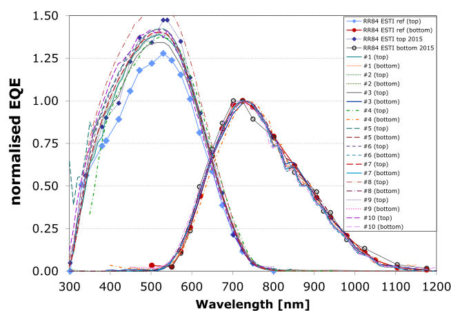
FIGURE 9 Normalised EQE of RR84 (nominally bottom-limited) for the laboratories that submitted the results. ESTI reference and the data measured before the DUTs pre-conditioning in 2015 are shown, too. The lines connecting ESTI measured points are only shown to help the reader's eye and do not represent any interpolation nor real data [Colour figure can be viewed at wileyonlinelibrary.com ]
