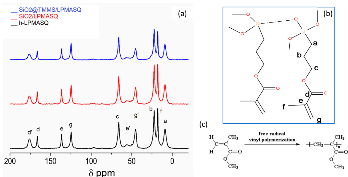
Figure 8. (a) ^{13}\text{C} CPMAS spectra of h-LPMASQ (black line), SiO 2 /LPMASQ (red line) and SiO 2 @TMMS/LPMASQ (blue line). The LPMASQ structure with C labeling and the polymerization scheme [68] are shown in figures (b) and (c), respectively.
