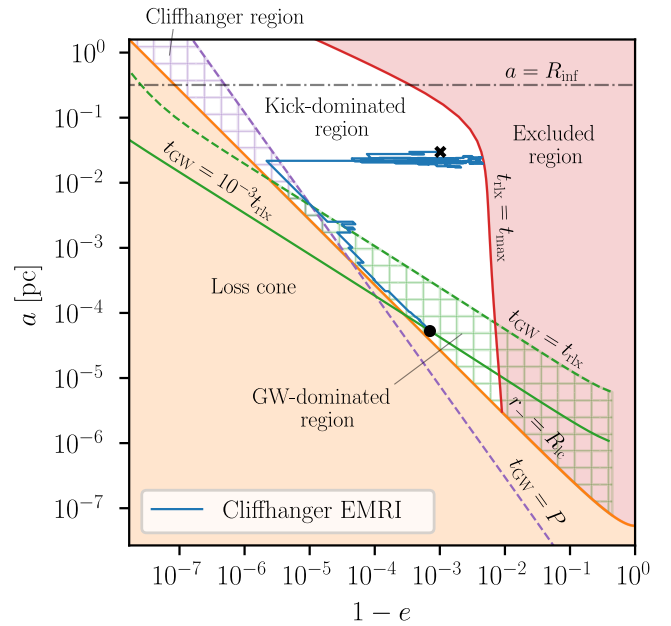
Fig. 3. Example of a cliffhanger EMRI orbit in the (1 - e, a) plane. The cliffhanger region is filled with a purple grid, and it is delimited by the purple dashed line and the orange solid curve (see Fig. 1 for the meaning of the other elements). The sharp tightening of the orbit at the passage inside the cliffhanger region occurs during a single pericentre passage. Here we set M_\bullet = 10^5 M_\odot .
