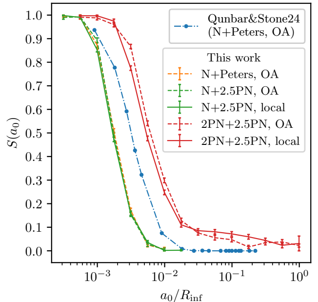
Fig. 13. Function S(a_0) given different assumptions on the dynamics and treatment of two-body relaxation. For the dynamics, we distinguish between Newtonian (N) or PN evolution of the system, and between employing the equations detailed in Peters (1964) or the 2.5PN term to treat loss of energy and angular momentum due to GW emission. Instead, two-body relaxation can be accounted for using the orbit-averaged approximation (indicated with OA), or locally. In all cases M_\bullet = 3 \times 10^5 M_\odot and the MBH is surrounded by a distribution of m_\star = 1 M_\odot stars only.
