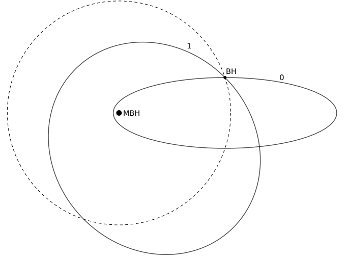
Fig. 6. Sketch depicting an example orbit change following our orbit-averaged procedure. The stellar-mass BH, initially on the orbit labelled 0, is kicked when r = a , and ends on the orbit labelled 1. Both orbits have the same semi-major axis a , but different eccentricities. The dashed circle represents a circular orbit with radius a . In this example there is no way to rotate either orbit around the focus occupied by the MBH such that the pericentre or apocentre of orbit 0 crosses orbit 1 at any point. Thus, neither pericentres nor apocentres are good spots to employ our orbit-averaged procedure. We note that the eccentricities of these example orbits are much lower compared to the ones investigated in this work. Moreover, the difference between subsequent orbits is much exaggerated here.
