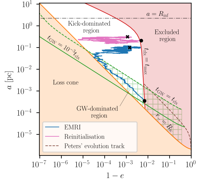
Fig. 8. Two examples of orbit evolution in the (1 - e, a) plane. The blue line shows the formation of an EMRI that is missed by our standard definition, and requires the correction described in the text to be rightfully counted. The pink line instead shows a regular reinitialisation. We also plot the evolution line of an orbit that passes through the minimum of the t_{\text{GW}} = 10^{-3} t_{\text{rlx}} curve following Eq. (32) (dashed brown line). It can be seen that all orbits that cross into the excluded region while being in the GW-dominated region fall below this evolution line, meaning they will reach the solid green curve, as long as the stochastic kicks due to two-body relaxation are small (see Fig. 1 for the meaning of the other elements). Here we set M_\bullet = 4 \times 10^6 M_\odot .
