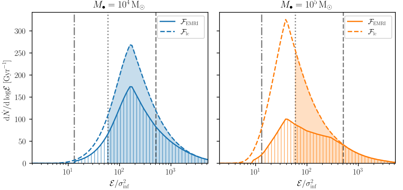
Fig. 15. Differential rate of EMRIs \mathcal{F}_{\text{EMRI}} (solid lines) and of EMRIs and DPs \mathcal{F}_{\text{cl}} (dashed lines) as functions of energy. The quantities refer to a nuclear cluster with M_{\bullet} = 10^4 M_{\odot} that has relaxed for 580 kyr (left panel) and one with M_{\bullet} = 10^5 M_{\odot} that has relaxed for 11 Myr (right panel). We report for reference vertical lines at the values of \mathcal{E} such that r_c(\mathcal{E}) is 0.1 R_{\text{inf}} (dash-dotted), 0.01 R_{\text{inf}} (dotted) and 0.001 R_{\text{inf}} (dashed). The colour-filled area of \mathcal{F}_{\text{cl}} gives the classical EMRI rate at r_c(\mathcal{E}) > 0.01 R_{\text{inf}} , to be compared with the hatched area of \mathcal{F}_{\text{EMRI}} over the full energy range. Apparent areas in the plot are proportional to the various integrals of the form \int d\mathcal{E} \mathcal{F} .
