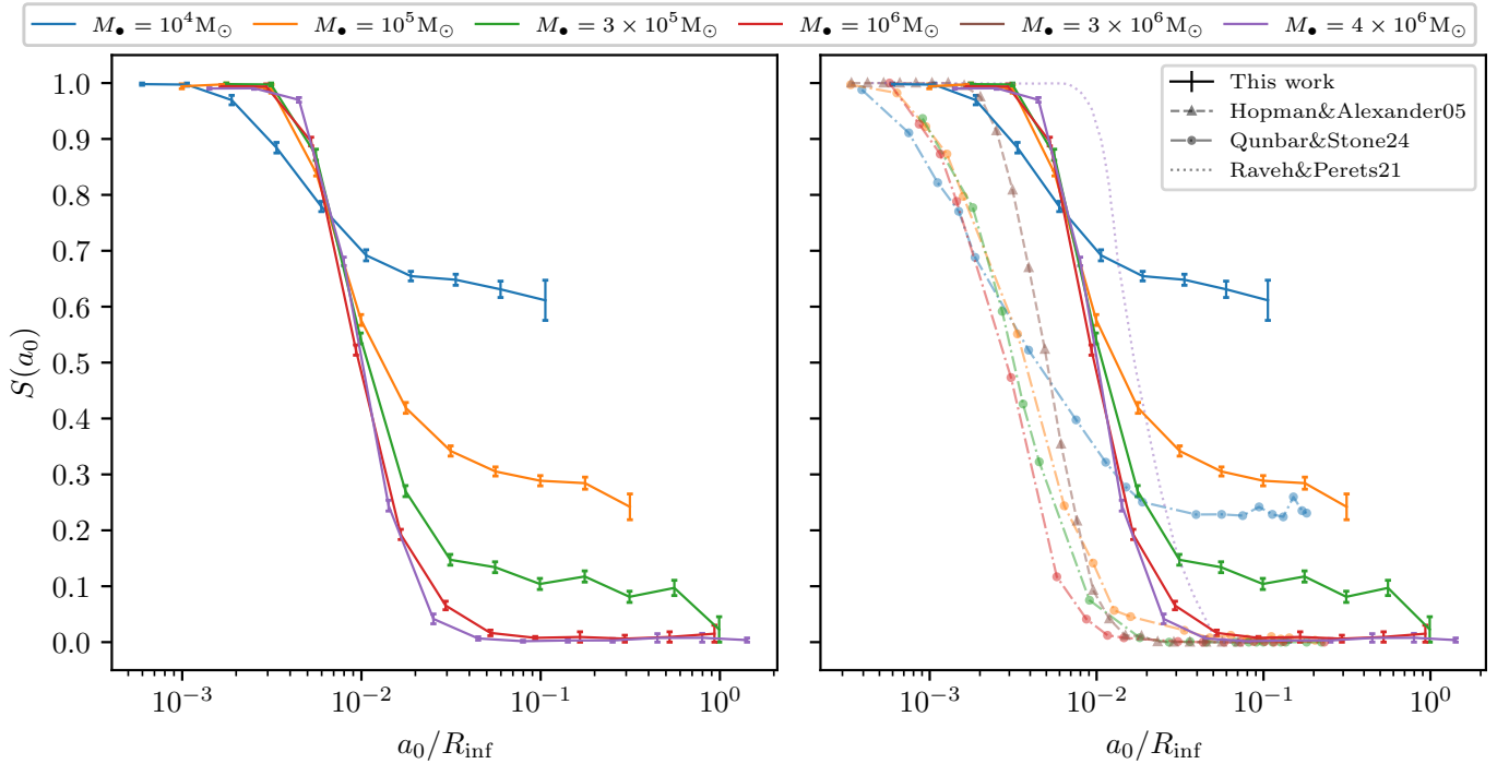
Fig. 9. Function S(a_0) for different M_* scenarios. The bars display 1\sigma uncertainty. The panel on the left displays our results only, while that on the right compares them with those from other works. We note that the other works make different assumptions, both with respect to our work and to each other.
