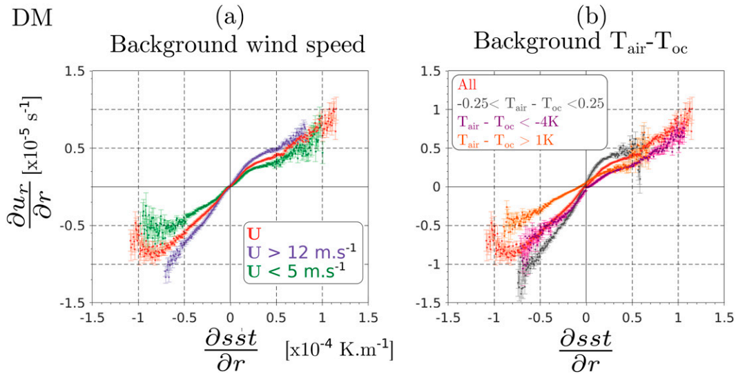
FIG. 3. As in Fig. 2a, with the discrimination of the data based on (a) background wind speed and (b) background air–sea temperature difference. In both panels, the red lines and points represent the binned distributions based on the full dataset and are strictly the same. In (a), the green and violet colors represent the data with the background wind speed lower than 5 \text{ m s}^{-1} and greater than 12 \text{ m s}^{-1} , respectively. In (b), the gray line shows data with a near-neutral stability, while the purple and orange colors are used for very unstable and very stable conditions, respectively, as indicated in the legend.
