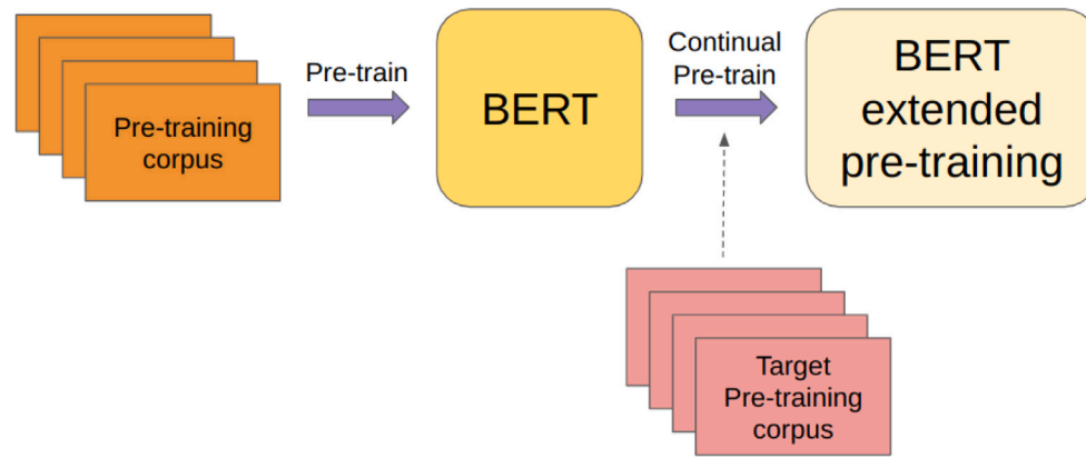
Fig. 5. Knowledge Injection with random masking.
