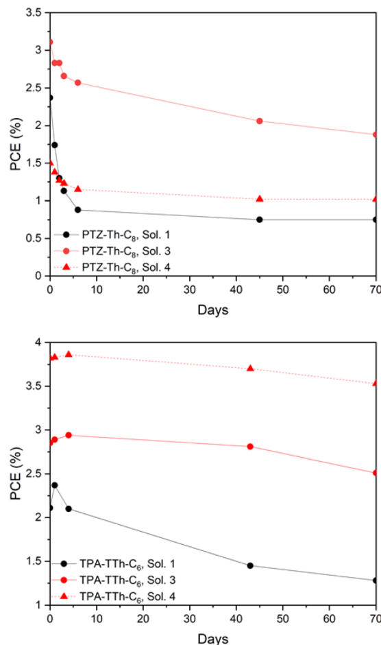
Fig. 9 PCE of PTZ-Th-C 8 (top) and TPA-TTh-C 6 (bottom) sensitized DSSCs in combination with CDCA as a co-adsorbent, filled with solutions 1, 3 and 4 (recordings up to 70 days from the initial cell assembly) recorded under AM1.5G irradiation.
