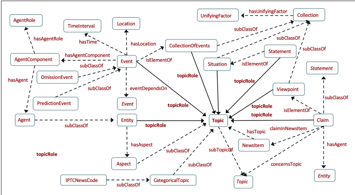
Figure 1. Synoptic view of the main classes and relations in our formal model of news classification.
