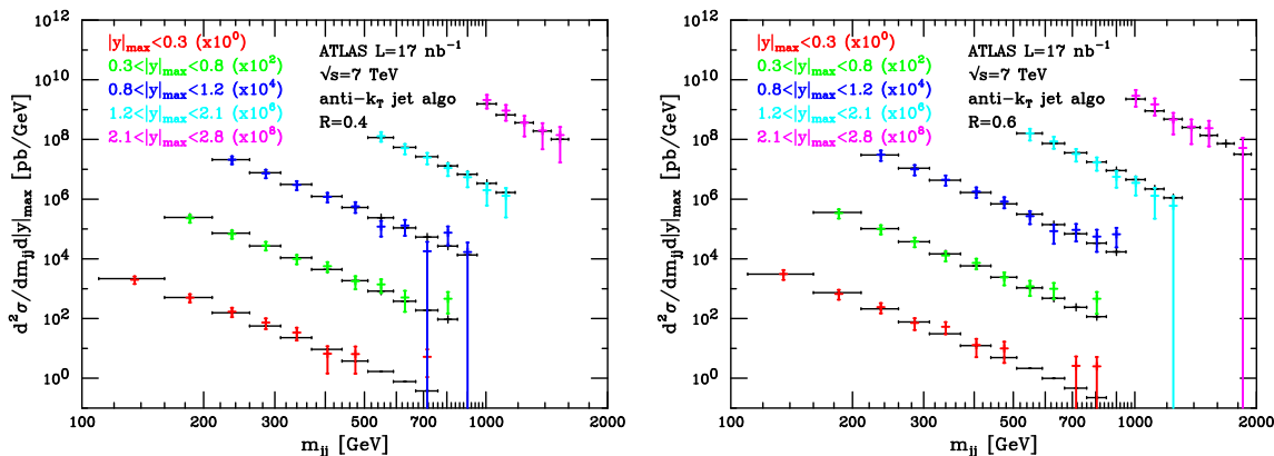
Figure 26. Predictions and experimental results for the double-differential inclusive jet cross section as a function of the dijet mass m_{jj} of the two leading jet pair, for different bins in |y|_{\max} , the maximum absolute rapidity of the two jets. The cuts of eq. (4.4) are imposed on the two leading jets. Black horizontal lines are the POWHEG+PYTHIA theoretical results (with errors). Coloured vertical bars describe the experimental data from ATLAS (systematic and statistical errors added in quadrature) [1]. Jets are recombined using the anti- k_T algorithm with R = 0.4 in the left plot, and R = 0.6 in the right one. Data are shown from top to bottom in order of decreasing rapidity.
