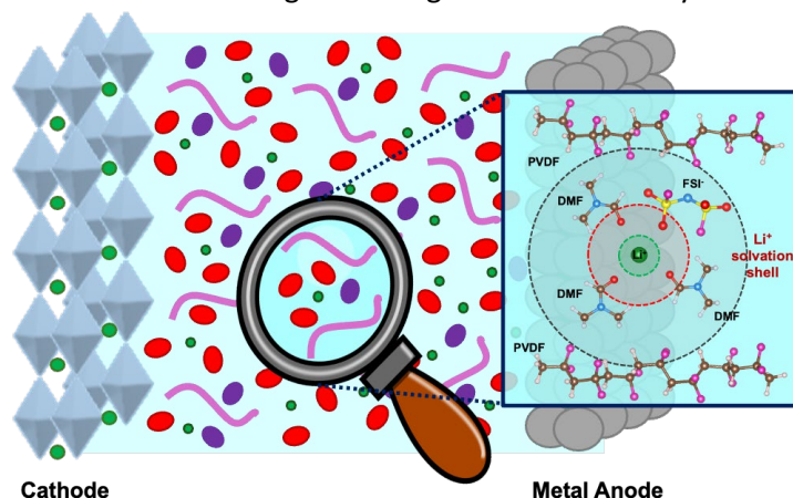
Figure 1. Li-ion solvation shell in PVDF-based quasi-solid electrolytes.
