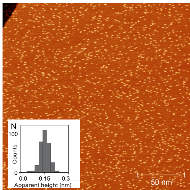
Fig. 3. STM image of Ta 8 clusters deposited and measured on Pt(111) at room temperature (0.04 clusters/nm 2 ). The height histogram (inset) clearly indicates that exclusively single-layer high clusters are formed, indicating monodisperse deposition. The clusters do not preferentially decorate the step in the upper left, pointing to their immobility at this temperature. Imaging parameters: 1.5 V, 0.3 nA.
