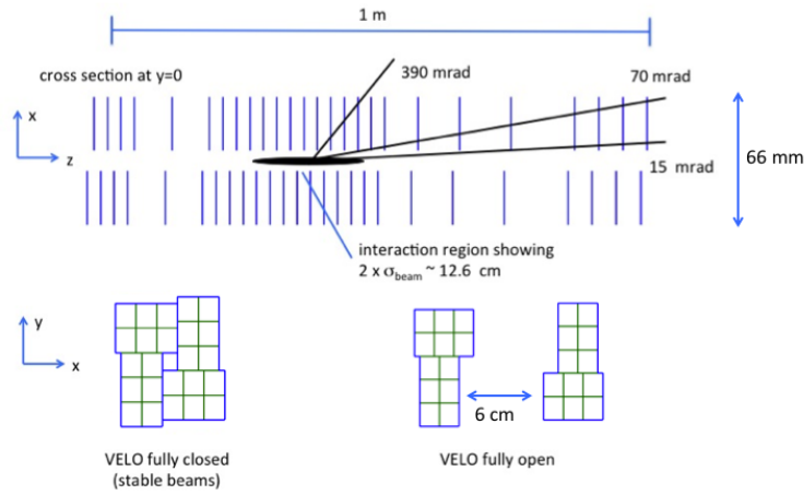
FIGURE 2.4: Layout scheme of the new VELO detector.
