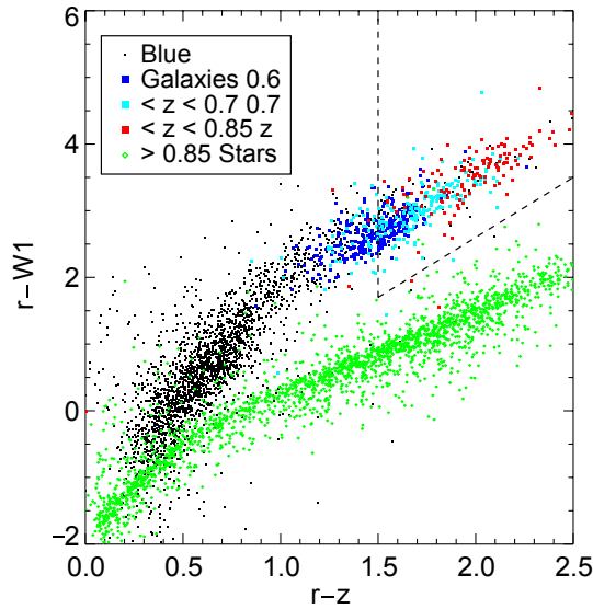
Figure 3.6: An optical/near-infrared color-color diagram for galaxies observed by both DECcam and WISE in the COSMOS field, where highly accurate 30-band photometric redshifts are available and used to label the points shown. In this and subsequent figures, r indicates DECcam r -band AB magnitude, z indicates DECcam z_{AB} , and W1 indicates WISE 3.4 \mu\text{m} AB magnitude. Galaxies with LRG-like spectral energy distributions also having z > 0.6 are indicated by points color-coded according to their redshift, whereas small black points indicate blue galaxies at all redshifts. The dashed lines indicate the borders of our LRG selection box; our baseline sample assumes that objects above and to the right of these lines that also have magnitude z_{AB} < 20.46 will be targeted by DESI as high-redshift LRGs.
